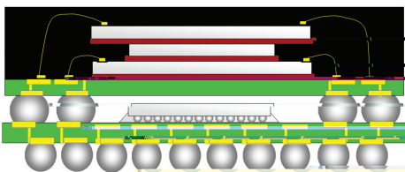
TFBGA-PoPt-SD3 + fcVFPGA-PoPb
